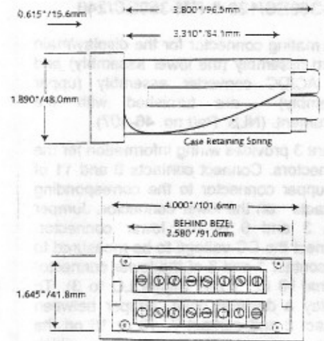
Figure 2. Terminal Block Config.
