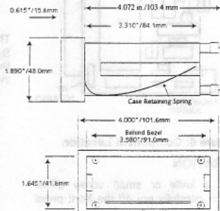
Figure 1: Card-Edge Configuration
